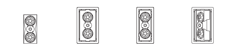
In-Room Monitor 7 1/2" x 16 1/2" x 9 1/2" 18.5 x 42.3 x 22.8 In-Wall/4 Monitor 10 1/2" x 19 x 3 7/8" 27.3 x 48.3 x 9.9 In-Wall/6 Monitor 8 1/2" x 19 x 5 7/8" 20.8 x 48.3 x 15 In-Ceiling/6 Monitor 10 1/2" x 19 x 5 7/8" 27.3 x 48.3 x 15
