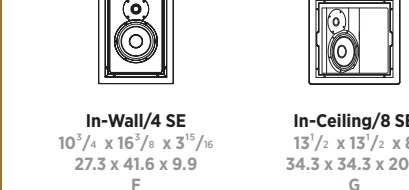
In-Wall/4 SE 10 1/2" x 18 1/2" x 9 1/2" 27.3 x 47.5 x 9.9 In-Ceiling/8 SE 13 1/2" x 13 1/2" x 8 1/2" 34.3 x 34.3 x 20.3
