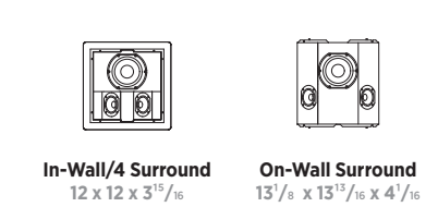
In-Wall/4 Surround 12.12 x 3 7/8" 30.4 x 30.4 x 9.9 On-Wall Surround 12 1/2" x 13 1/2" x 4 1/2" 33.4 x 35 x 10.4
