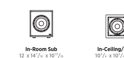
In-Room Sub 12 x 14 1/2" x 10 1/2" 30.4 x 36.6 x 27.4 In-Ceiling/8 Sub 10 1/2" x 10 1/2" x 7 1/2" 27.3 x 27.3 x 19.1
