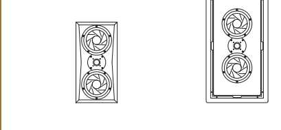
In-Room Monitor 9 1/2" x 19 1/2" x 12 1/2" 25.1 x 49.2 x 31.5 In-Wall/6 Monitor 13 1/2" x 26 x 5 7/8" 34.3 x 66 x 15
