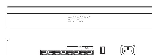
SE-8P4 8-Port Unmanaged Switch with 4 PoE or Up to 2 PoE+ (322 × 185 × 44 mm)
