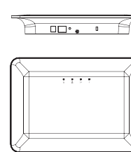
WX-1 802.11ac 3x3 Wireless AP, Plenum Rated (249 × 179 × 36 mm)
