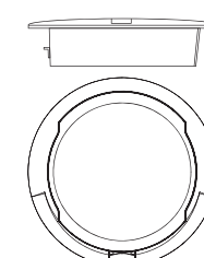
WK-2-C 802.11ac 3x3 Wireless AP, In-Ceiling (204 × 190 × 41 mm)
